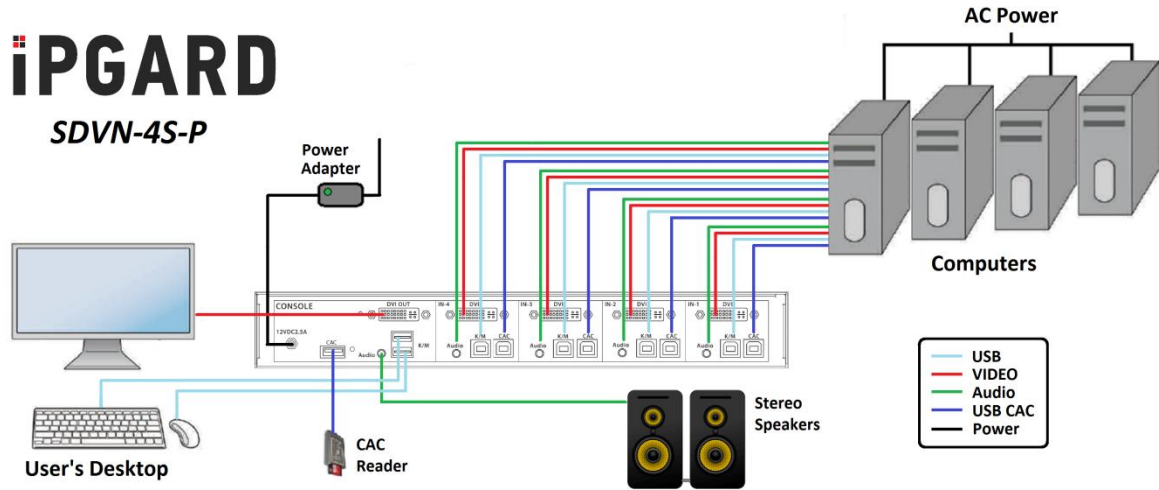
Figure 1: Standard Setup of 4-Port KVM TOE Installation
